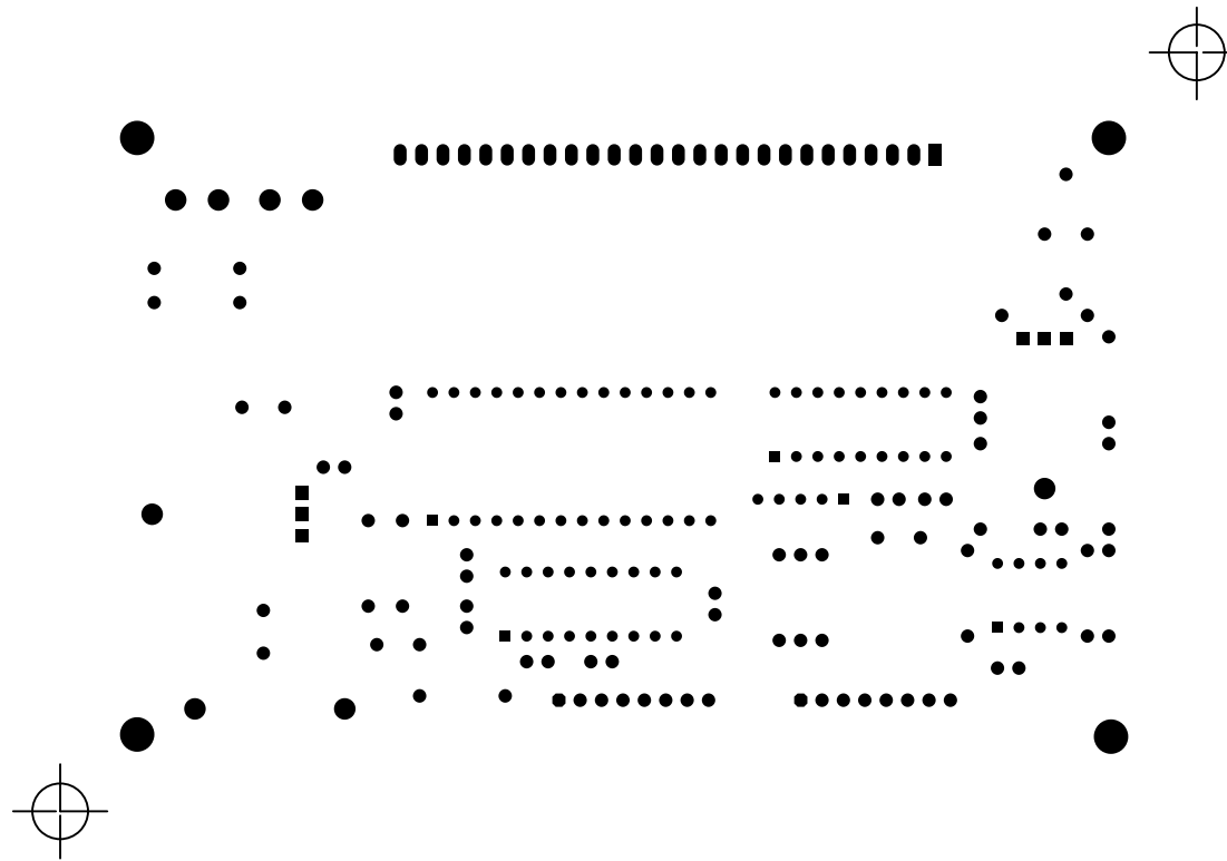
VFD 11 Digit Display Rev EB
